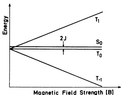
FIGURE 3 Magnetic field dependence of the radical ion pair singlet and triplet state energies ( J = exchange interaction energy). The observed magnetic field effects demonstrate that the hyperfine interaction coupling, inducing coherent S \rightleftharpoons T transitions in the radical pairs, is predominant.
