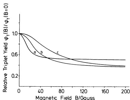
FIGURE 5 Magnetic field dependence of the relative triplet yield \phi_T(B)/\phi_T(B=0) from the ( ^2\text{D}^+ + ^2\text{A}^- ) radical pairs calculated with the sums of the hyperfine coupling constants \Sigma a_{D^+} \sim 24 G (for the bacteriochlorophyll radical) and \Sigma a_{A^-} \sim 32 G (for the bacteriopheophytine radical) and with k_S = k_T = k for a, k = 0.1 \times 10^9 \text{ s}^{-1} ; b, k = 0.5 \times 10^9 \text{ s}^{-1} ; c, k = 1.0 \times 10^9 \text{ s}^{-1} (exchange interactions J_{D,A} = J_{A,X} = 0 ).
